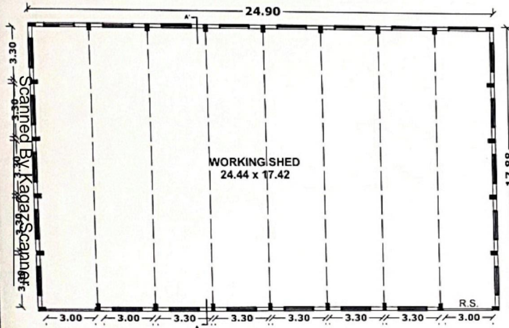
PLAN (SCALE-1:200)
